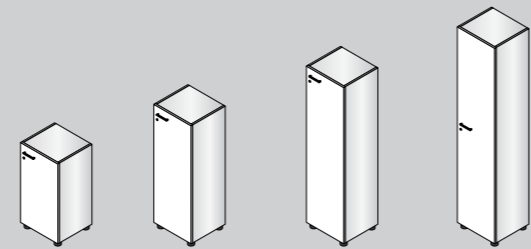
J4508C 45x41,4x83 h J4512C 45x41,4x121,4 h J4516C 45x41,4x159,8 h J4520C 45x41,4x201,4 h
