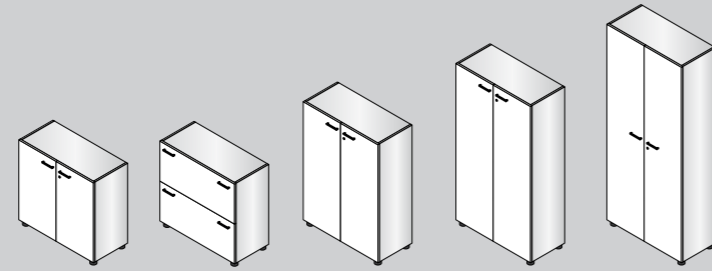
J9008C 90x41,4x83 h J9008CL 90x41,4x83 h J9012C 90x41,4x121,4 h J9016C 90x41,4x159,8 h J9020C 90x41,4x201,4 h
